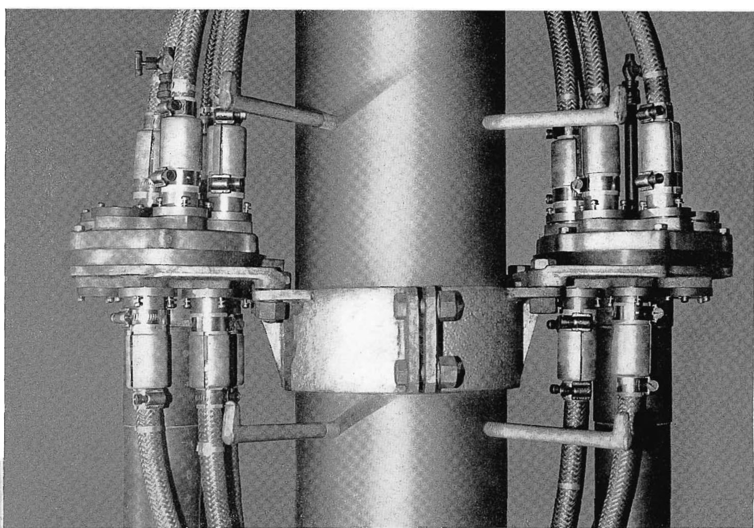
Junction boxes which connect individual feed lines to the rigid coaxial lines shown mounted on supporting pole for Super Turnstile. Junction boxes for Super Gain elements mounted within tower.
