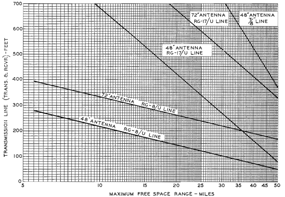
FIG. 4 (above). Chart showing typical ranges of BTL-1A link.
