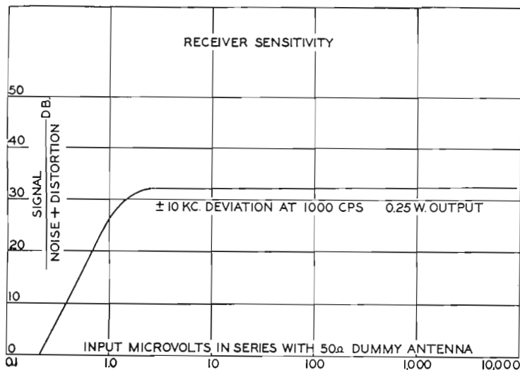
FIG. 14. Receiver sensitivity.
