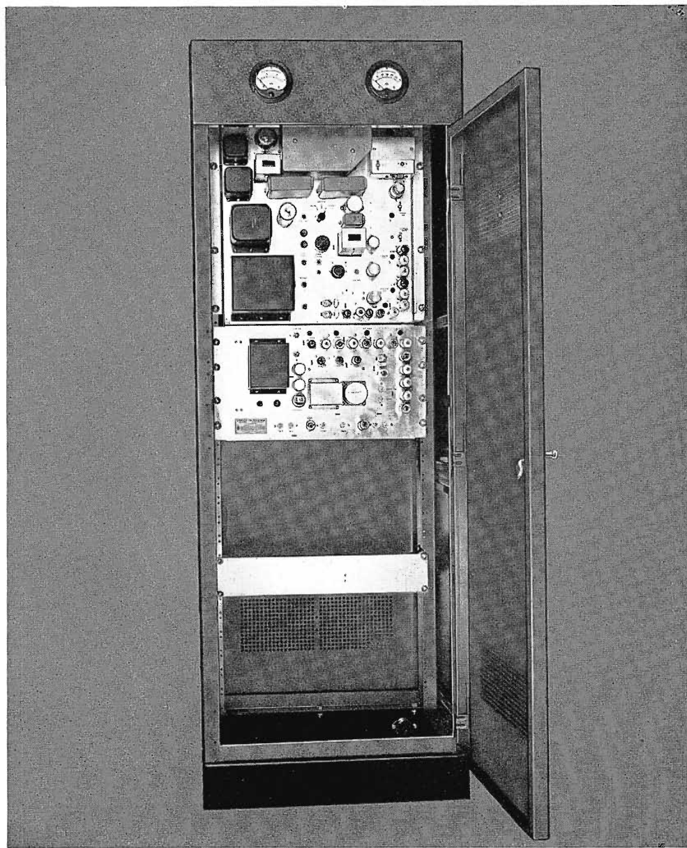
FIG. 25. RCA's two way radio systems are built to the same exacting standards as its broadcasting and television equipment. Shown above is a 70 watt station transmitter and receiver with separate built-in power supplies. Cabinet can accommodate additional receiver for dual frequency operation.
