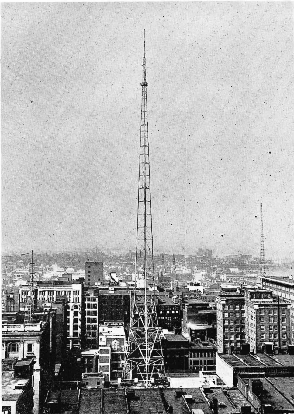
FIG. 8. View of the KSD-TV 3-bay RCA Super Turnstile Antenna and tower located atop the Post-Dispatch Building.
