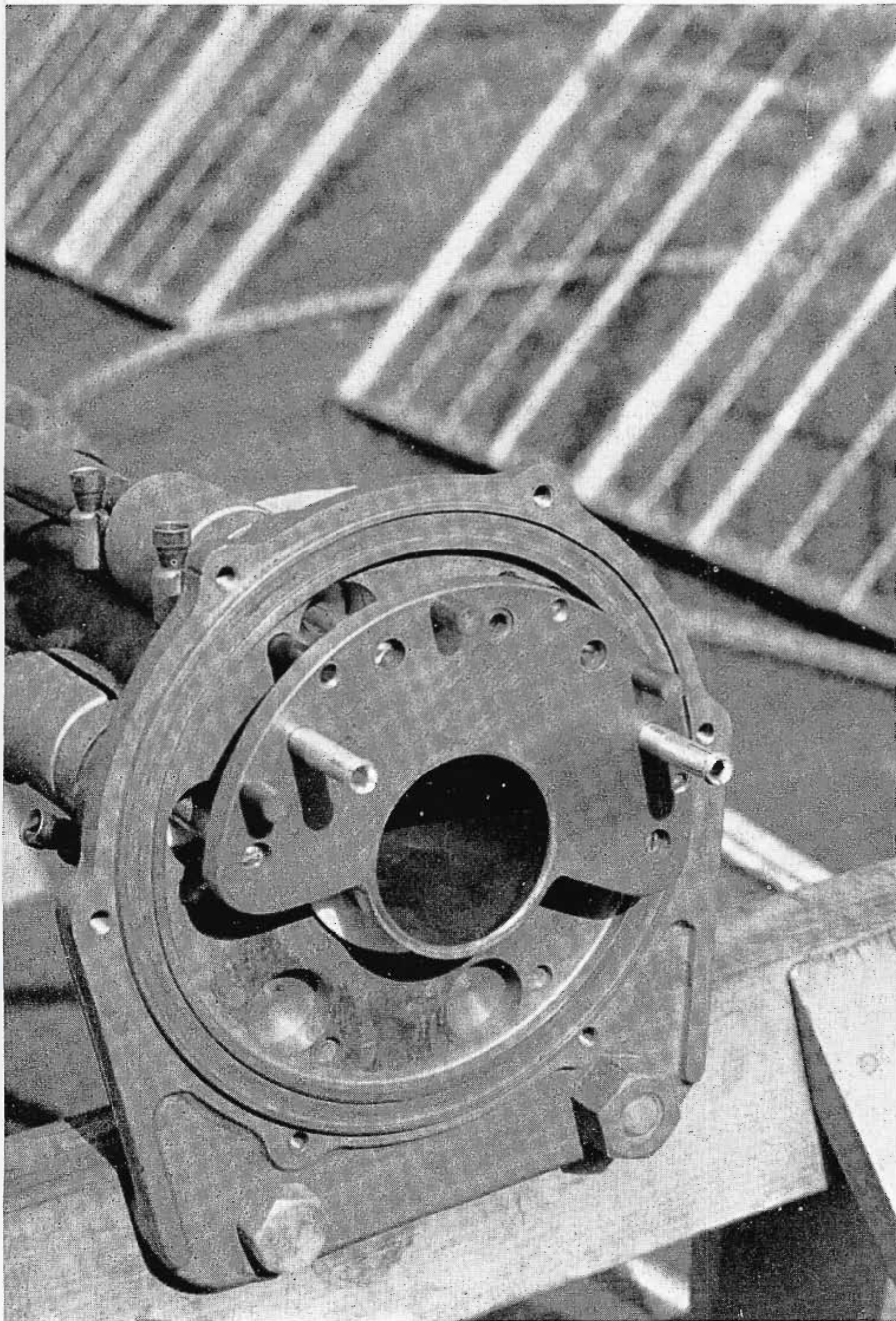
◀ Disassembled junction box shows the method of interconnecting feed lines to the main transmission line which is a 52-ohm air-dielectric coaxial line.
