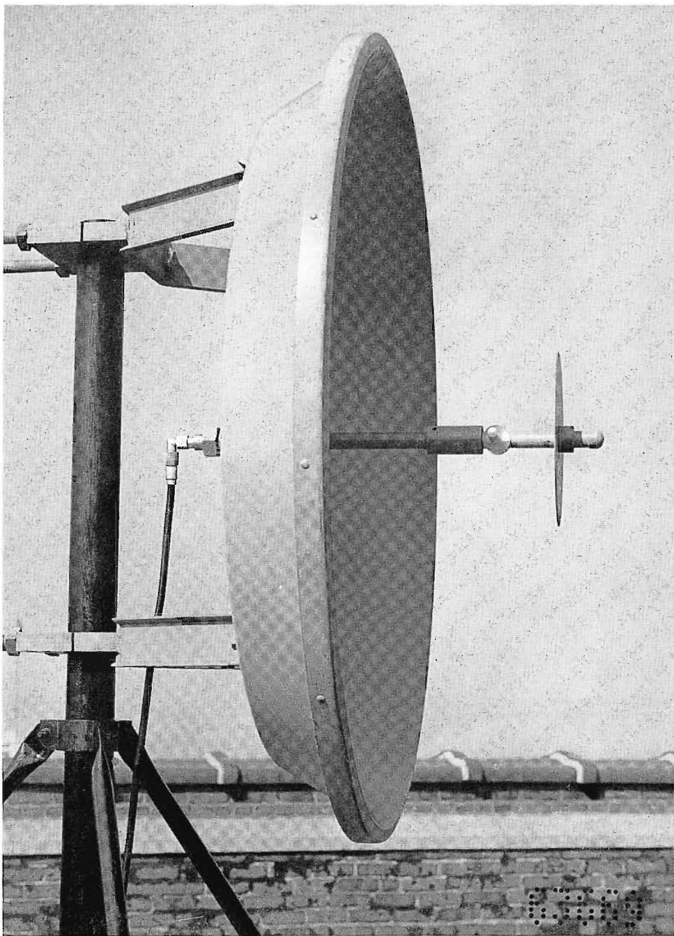
FIG. 2. Typical 48-inch parabolic reflector and antenna assembly. The antenna is fed by RG-17/U transmission line.
