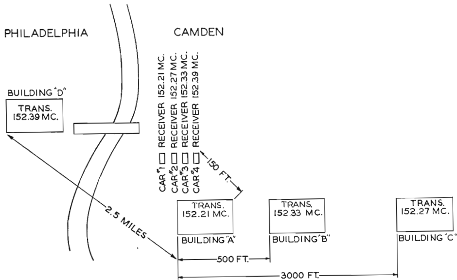
FIG. 5. Diagram shows location of mobile and land station during four channel test Number One.
