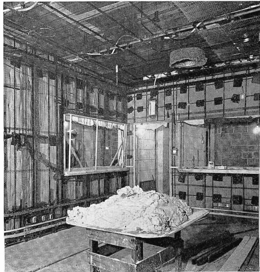
▲ FIG. 7. Perforated asbestos cement panels are used on three sides and plastered basket-weave pattern on fourth.
