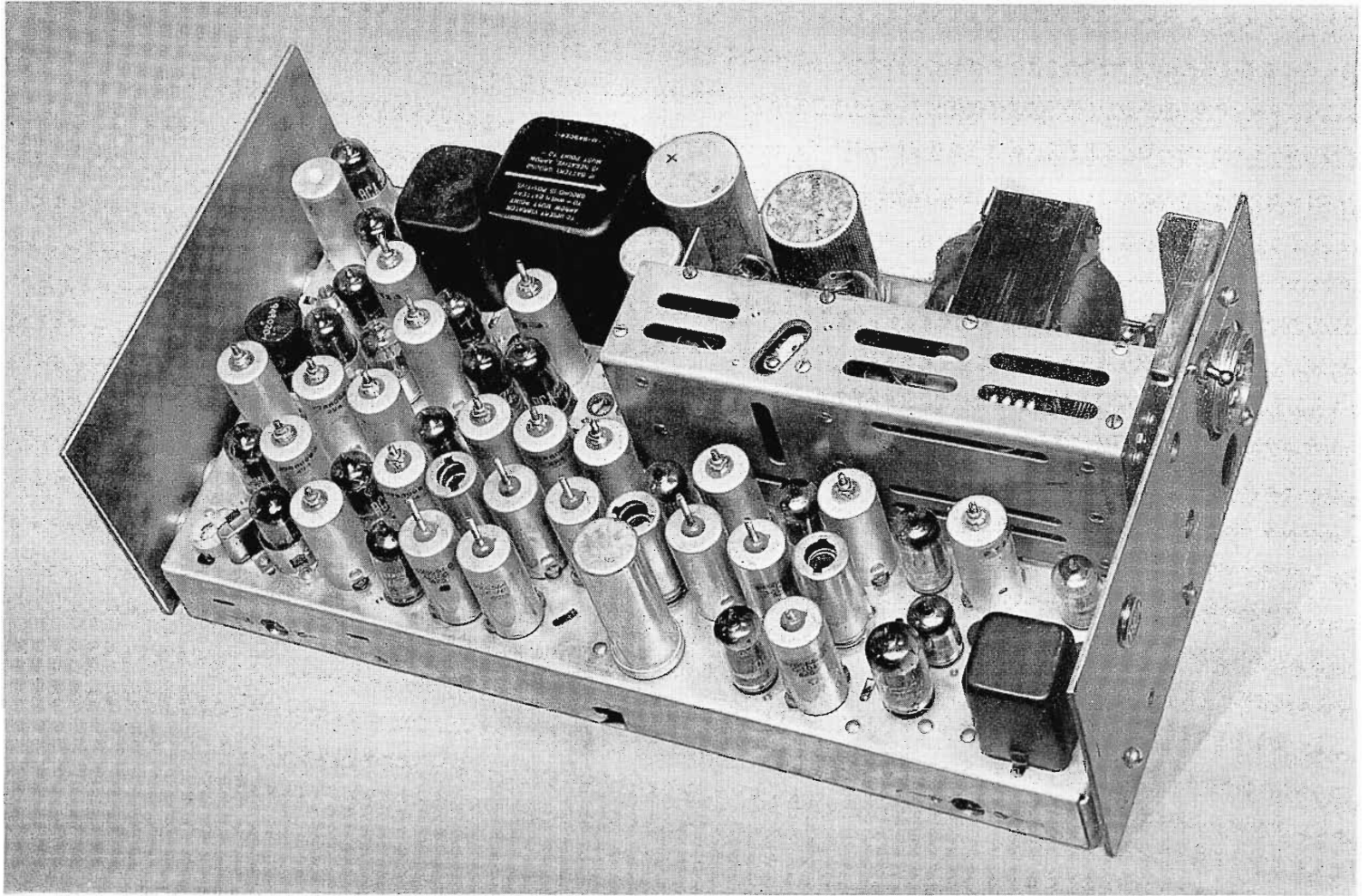
FIG. 1. The 15 watt RCA Carfone shown above, was the first adjacent channel two way radio equipment on the market. Completely open, accessible construction puts every component and every connection "on top". The unit can be removed for service in thirty seconds.
