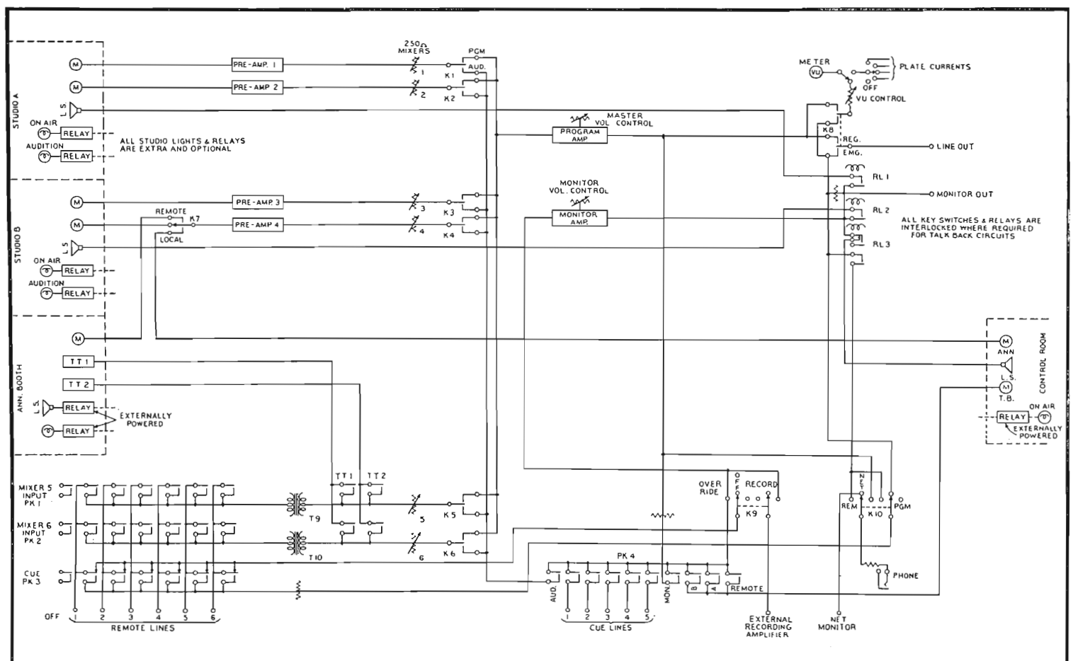
FIG. 1 (below). Simplified block diagram of 76-B5 Console.
