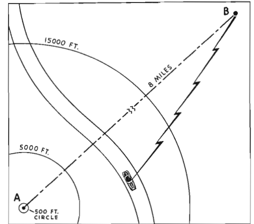
FIG. 2. Benefits of the Carfone's high selectivity are most effectively demonstrated where stations, which have overlapping areas of signal coverage, are assigned adjacent channels. Greater selectivity makes it possible for the RCA mobile equipment to maintain interference-free communications over a much greater area in the region of the overlap. Actual test showed that the RCA Carfone could operate within 500 feet of an adjacent channel station without interference while other equipment had interference radius of 5,000 to 20,000 feet. The new 30 watt Super-Carfone, shown below, operates efficiently within A FEW FEET of adjacent channel station.
