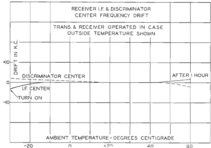
FIG. 17. Receiver intermediate-frequency drift.
