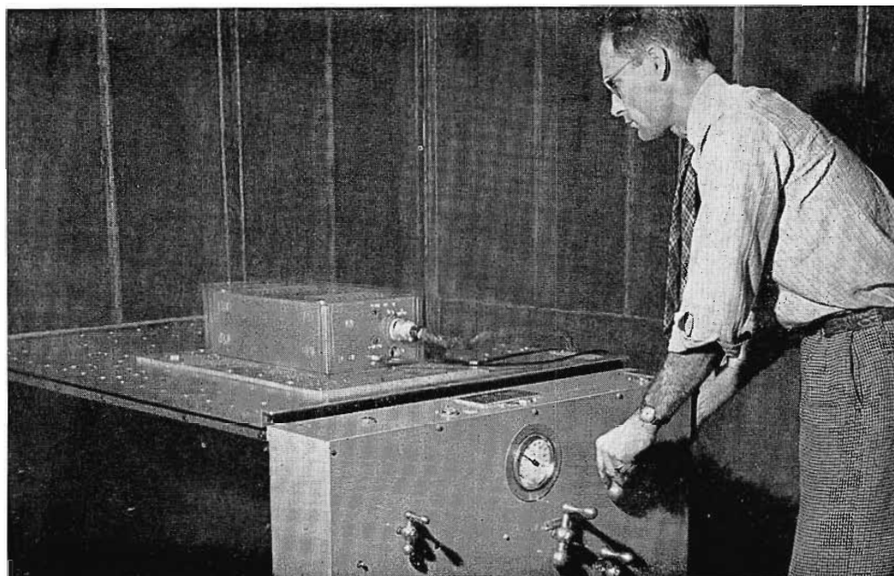
FIG. 24. To insure optimum performance under extreme conditions of temperature, humidity, and vibration, RCA engineers subjected the Carfone equipment to much tougher treatment than it has to take in actual practice. The Carfone passed tests illustrated (left). ICE TEST: -30 to +60 degrees; HUMIDITY TEST: 90 percent humidity at +60 degrees C. for several days; VIBRATION TEST: several hours of constant vibration in three planes with amplitude of \pm 1/32 inch at a frequency variation of 5 to 55 cycles per second.
