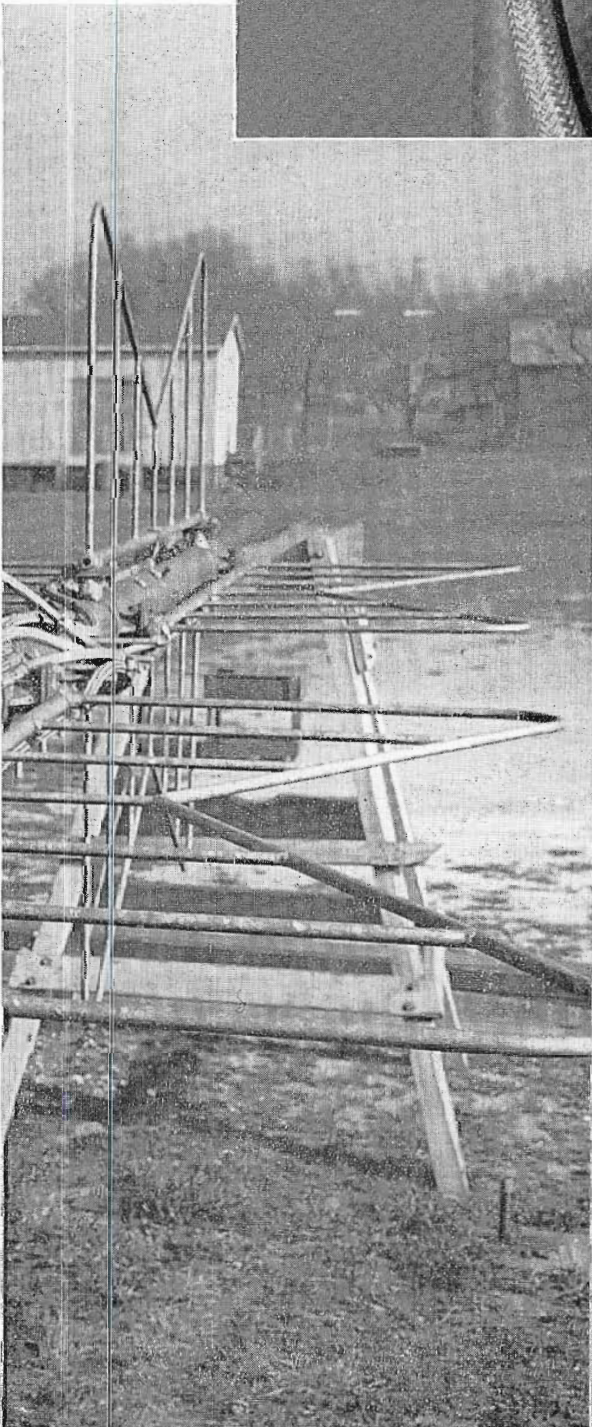
Junction boxes which connect individual feed lines to the rigid coaxial lines shown mounted on supporting pole for Super Turnstile. Junction boxes for Super Gain elements mounted within tower.
