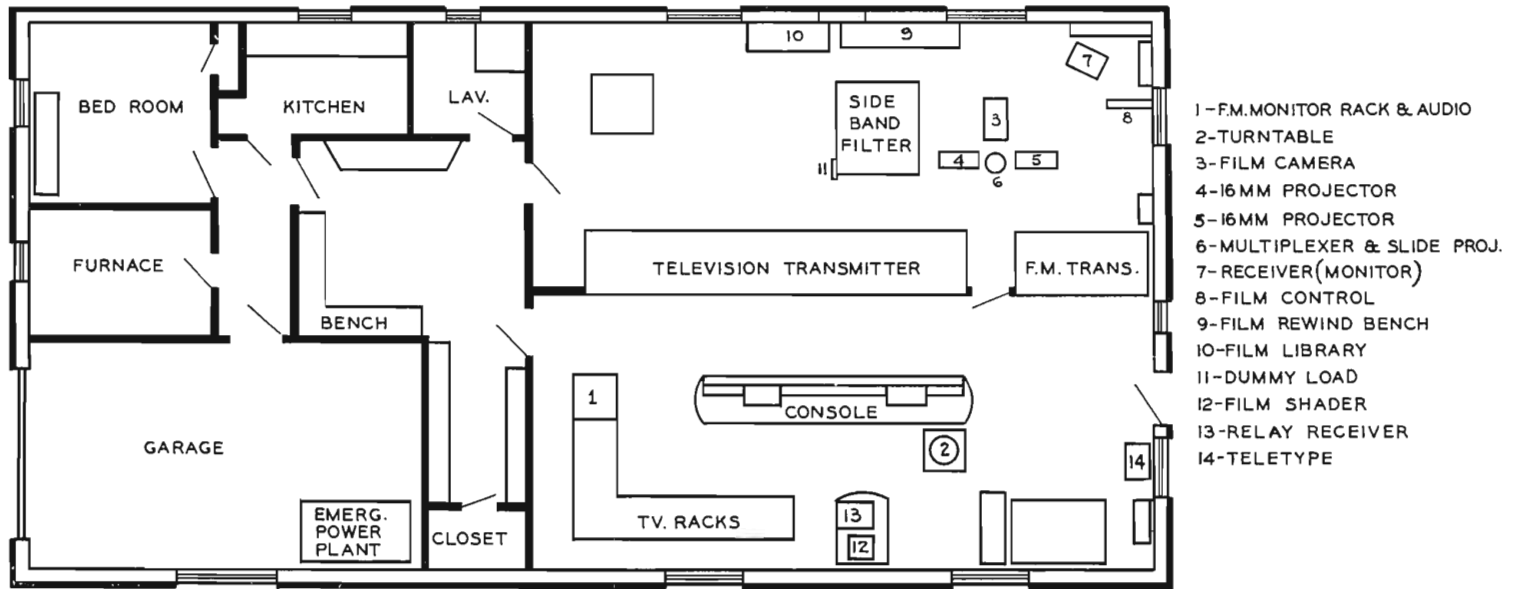
Diagram above is a floor plan layout of the WJAC-TV transmitter building. The transmitter console combines FM, TV and program control functions as described in the text.
