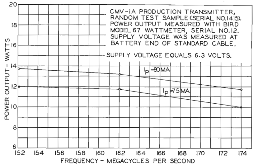
FIG. 22. Power output chart of transmitter random test sample.
