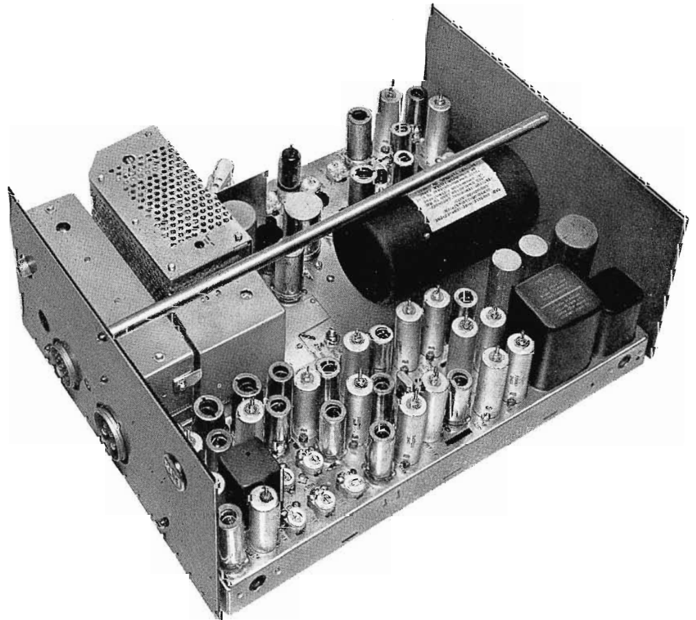
FIG. 3. The 30 watt RCA Super-Carfone, introduced recently, provides excellent performance in crowded metropolitan areas as well as farther out in the suburbs where the going is tough. Unique grounded-grid r-f input circuit provides high receiver sensitivity and simplified tuning.
