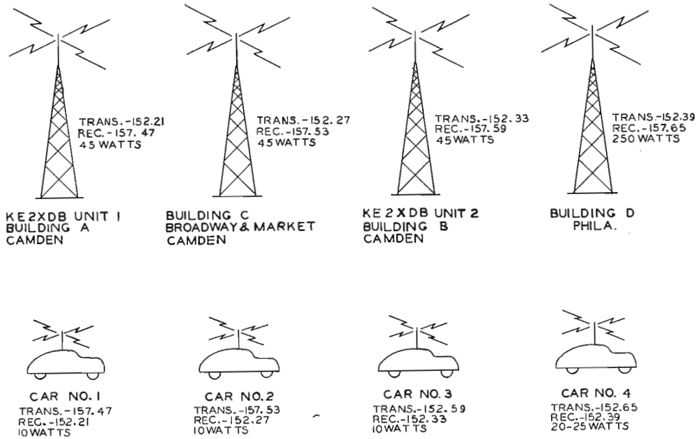
FIG. 4. Four separate stations transmitted on adjacent channels during the series of tests.
