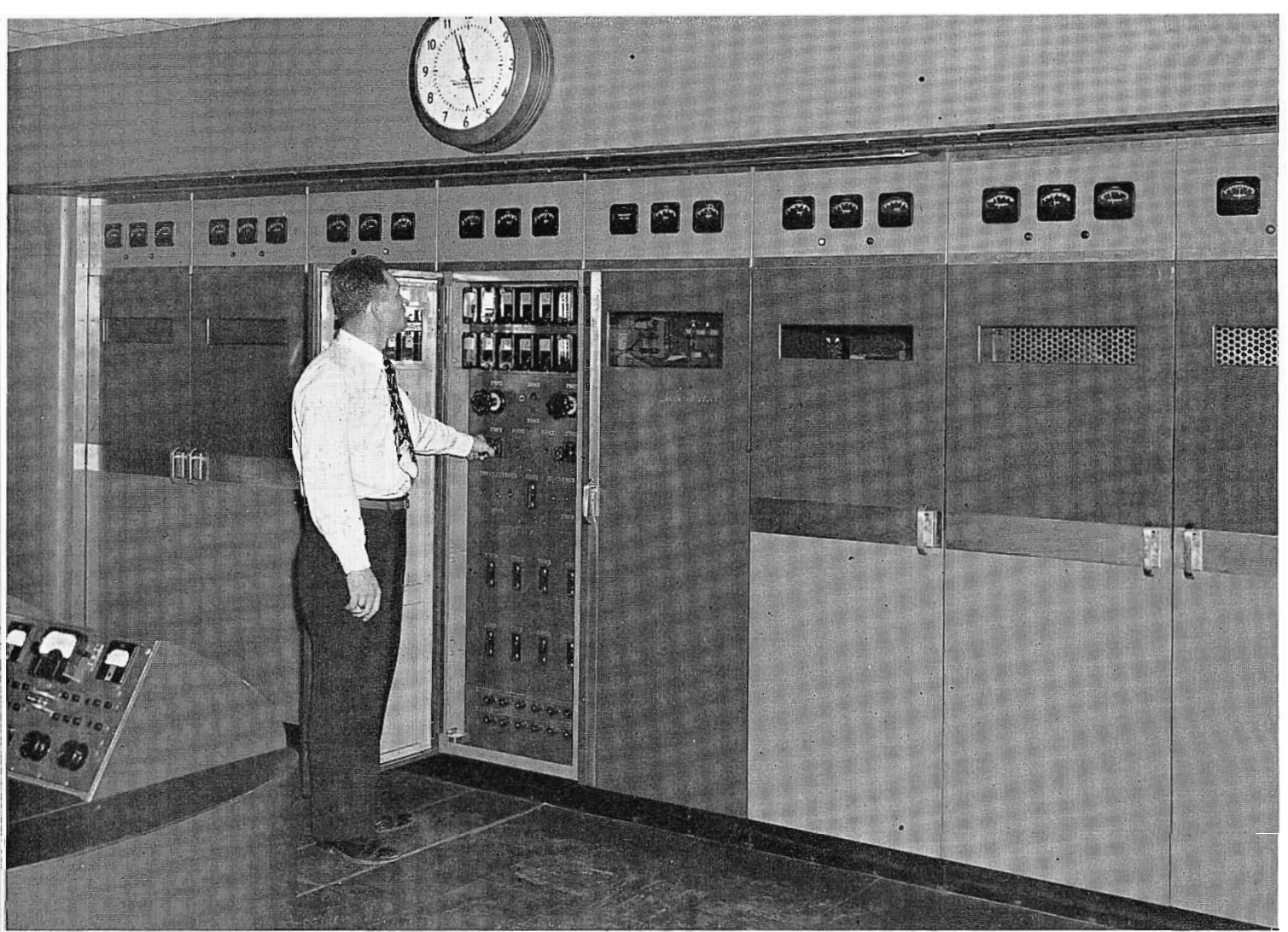
FIG. 9 (above). Front view of the TT-5A, RCA 5-kw transmitter which is flush-mounted in one side of the transmitter room. At left, part of the transmitter control console is visible.
