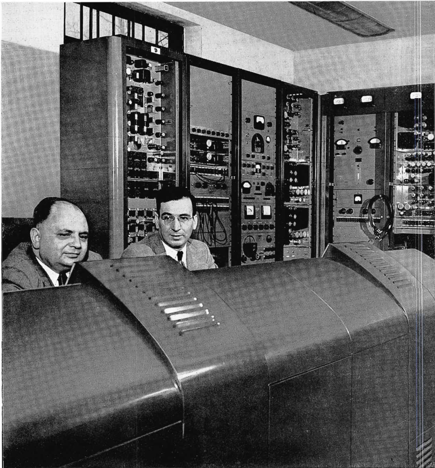
View from opposite side of transmitter room showing equipment racks arranged in one corner. Equipment consists of sync generator (left hand rack) audio and video patch panels, input and monitoring equipment, power supplies. Seated at the console with Nevin Straub is Ted Campbell, Assistant Chief Engineer.
