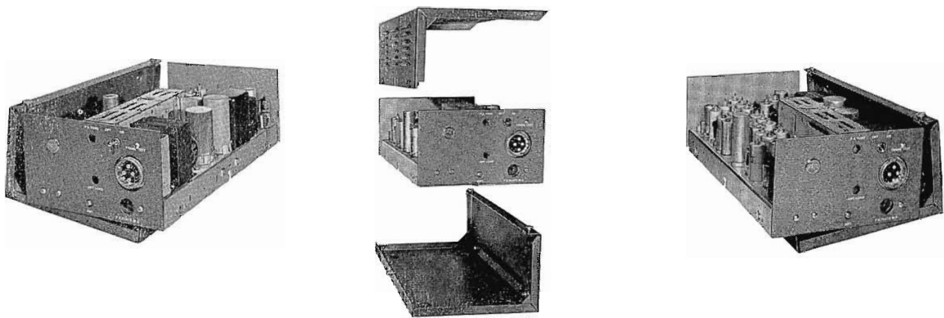
FIG. 23. The ingenious construction of the Carfone permits the widest choice of installation locations. The mounting base of the mobile equipment becomes one-half of the case. The cover becomes the top of the case forming "sandwich case" construction and providing such great flexibility as reversing the chassis 180 degrees without changing the position of the case plate or cover. This type of construction simplifies servicing, and requires no headroom as in drawer type cases. As shown at left, the chassis is ready for left-hand mounting; and for right-hand mounting at extreme right. Accordion view, in center, shows the construction of the chassis and housing.
