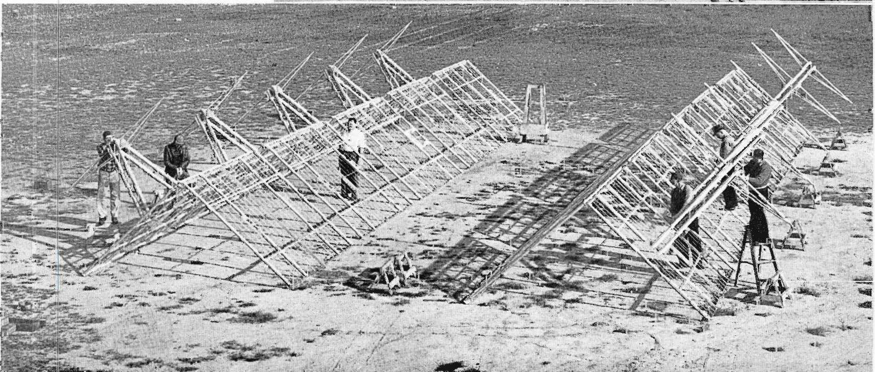
Channel 2 radiating elements being assembled on the screens prior to erection on the tower. Prefabrication of the screens and dipoles speeds erection.
