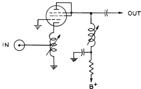
FIG. 11. Radio frequency amplifier in the first stage of the receiver.
