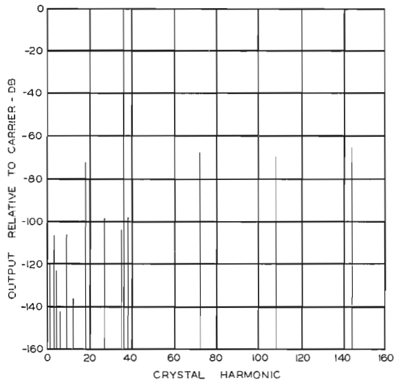
FIG. 21. Chart of spurious emissions of RCA Carfone transmitter, type CMV-1A, tuned to 158.31 mc.
