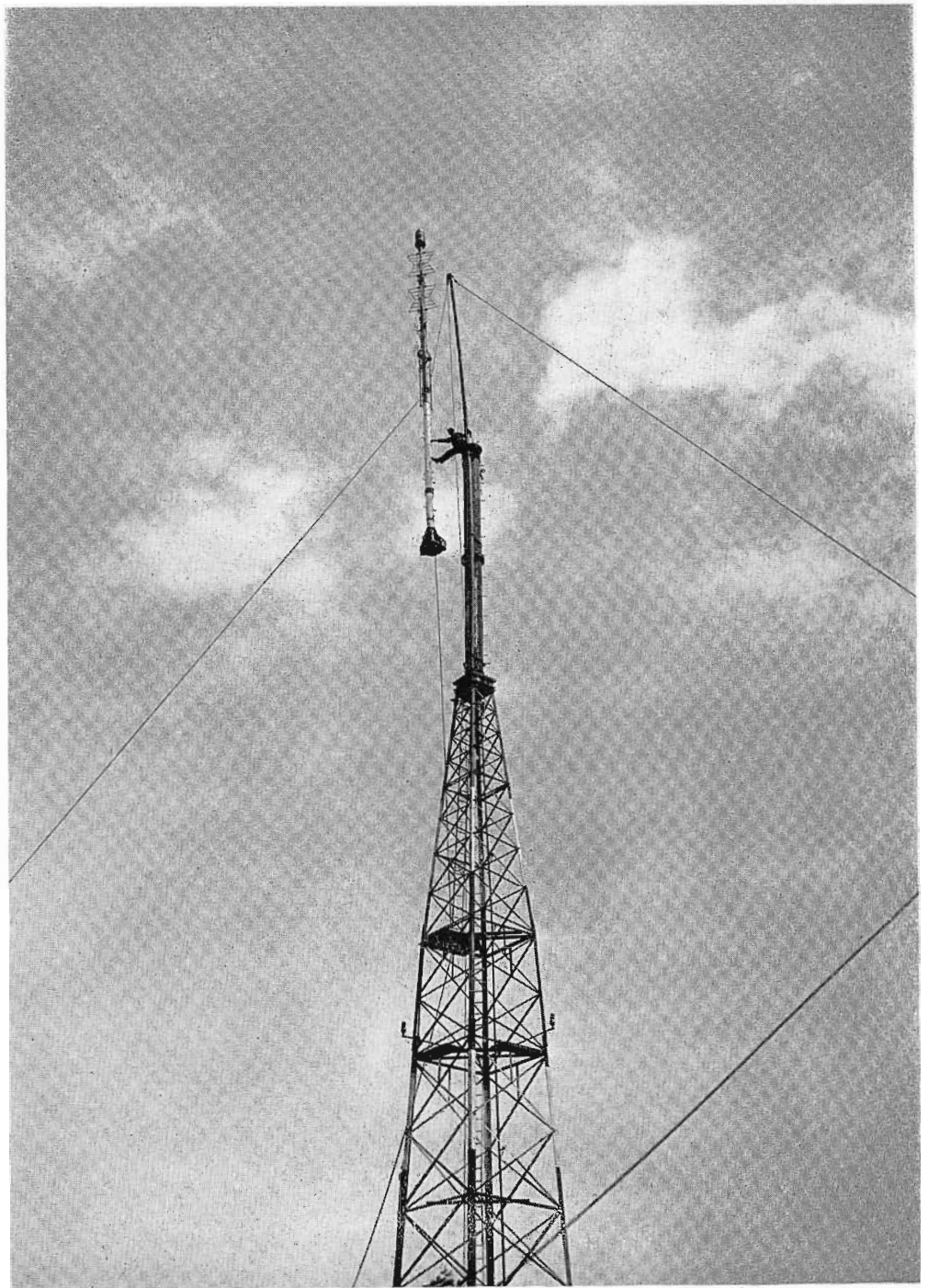
View of WJAC tower taken during erection of TV Super Turnstile on top the Pylon FM antenna.
