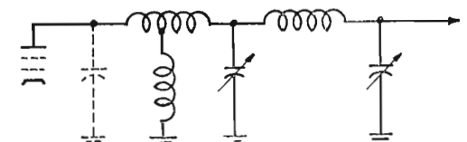
FIG. 20. Transmitter output filter circuit.
