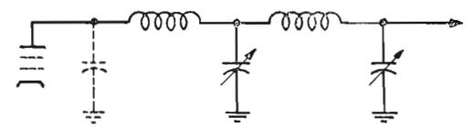
FIG. 19. Transmitter output circuit.
