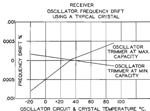
FIG. 18. Receiver oscillator stability.
