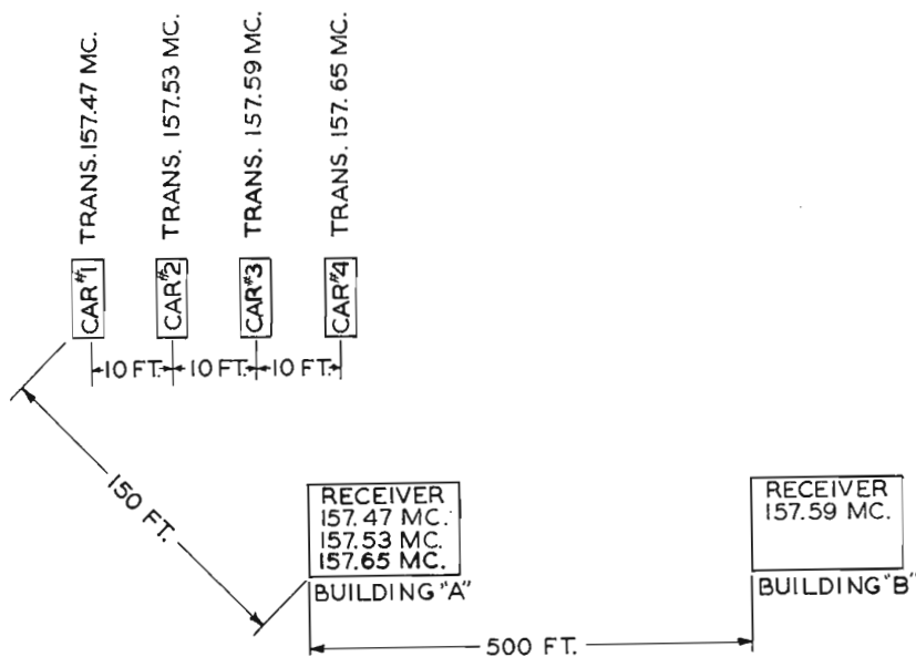
FIG. 5. Diagram shows location of mobile and land station during four channel test Number One.
