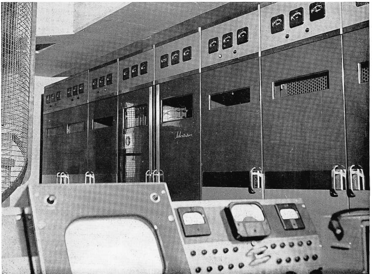
FIG. 15. View of PRF3-TV's 5-kw RCA Transmitter and Control Console as installed at Sao Paulo Bank Building.
