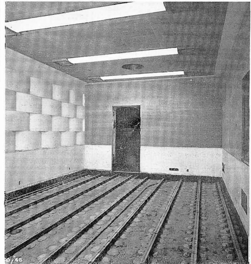
▼ FIG. 9. A floating floor resting on cork and spring supports helps provide "room-within-room" isolation. Wainscoting and trim are painted to harmonize with the wall surfaces.
