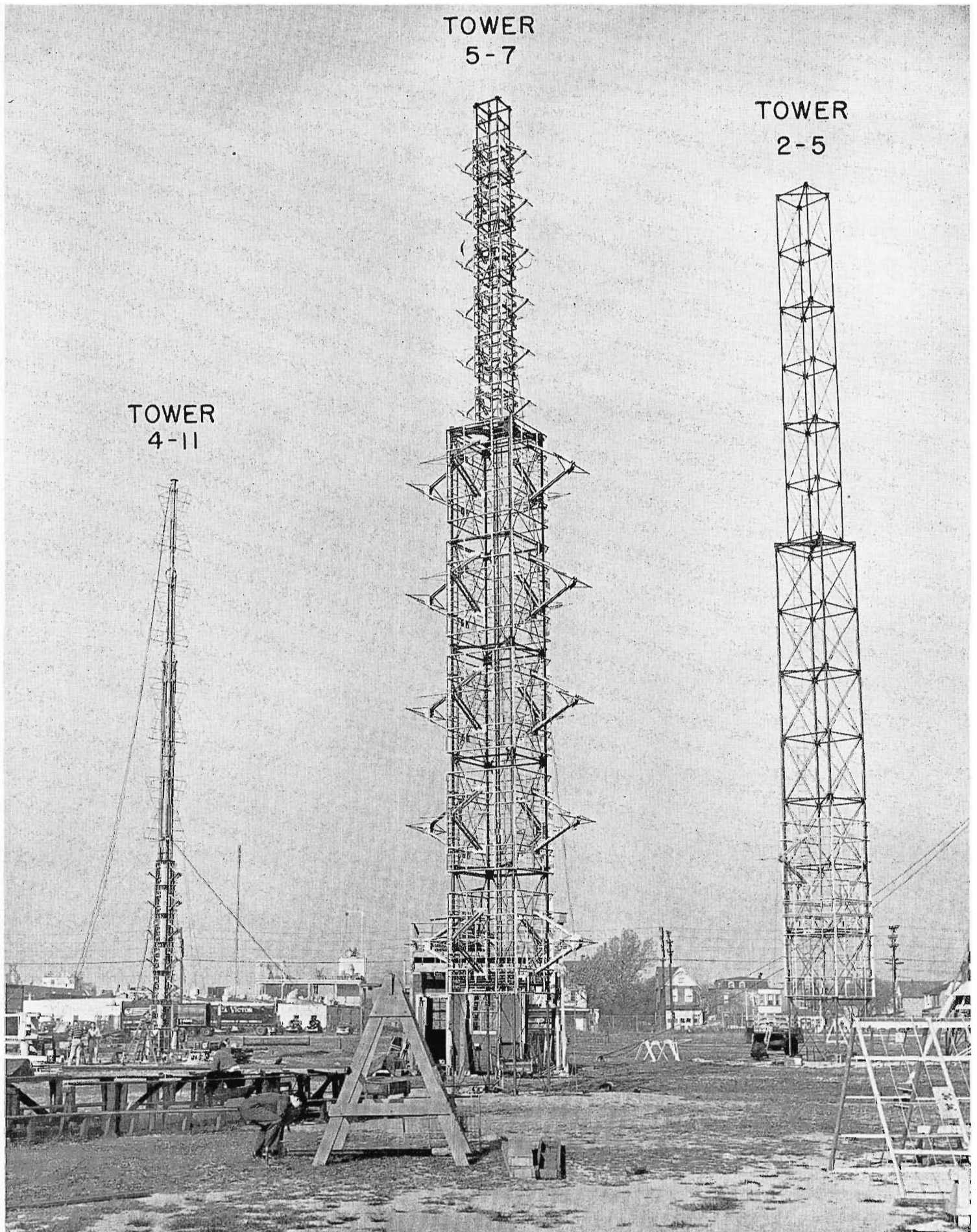
Photo above is a closeup of three of the four towers erected in Camden. The "5-7" tower in the foreground supports the elements for Channels 5 and 7, the "2-5" supports the elements for
