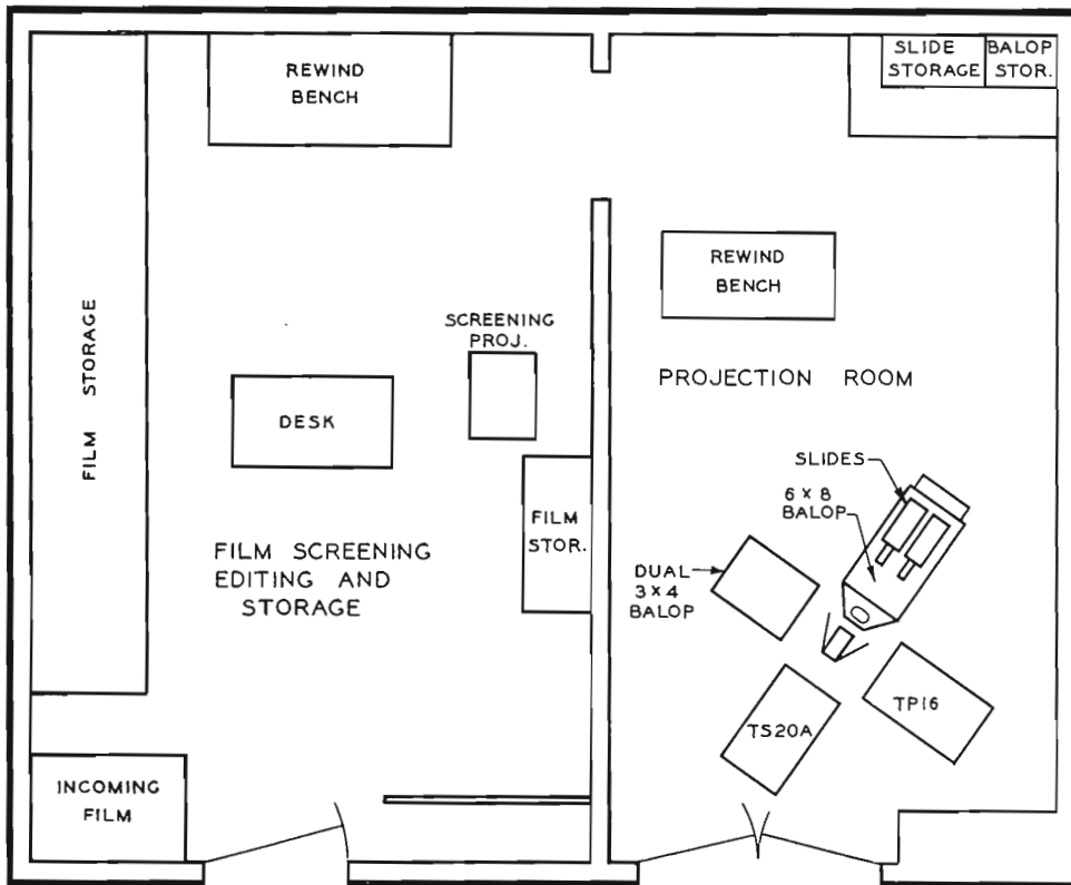
FIG. 4 (above). Floor plan layout of the KSD-TV Film Projection, Film Screening, Editing and storage facilities. Floor space occupied is approximately 600 square feet.
