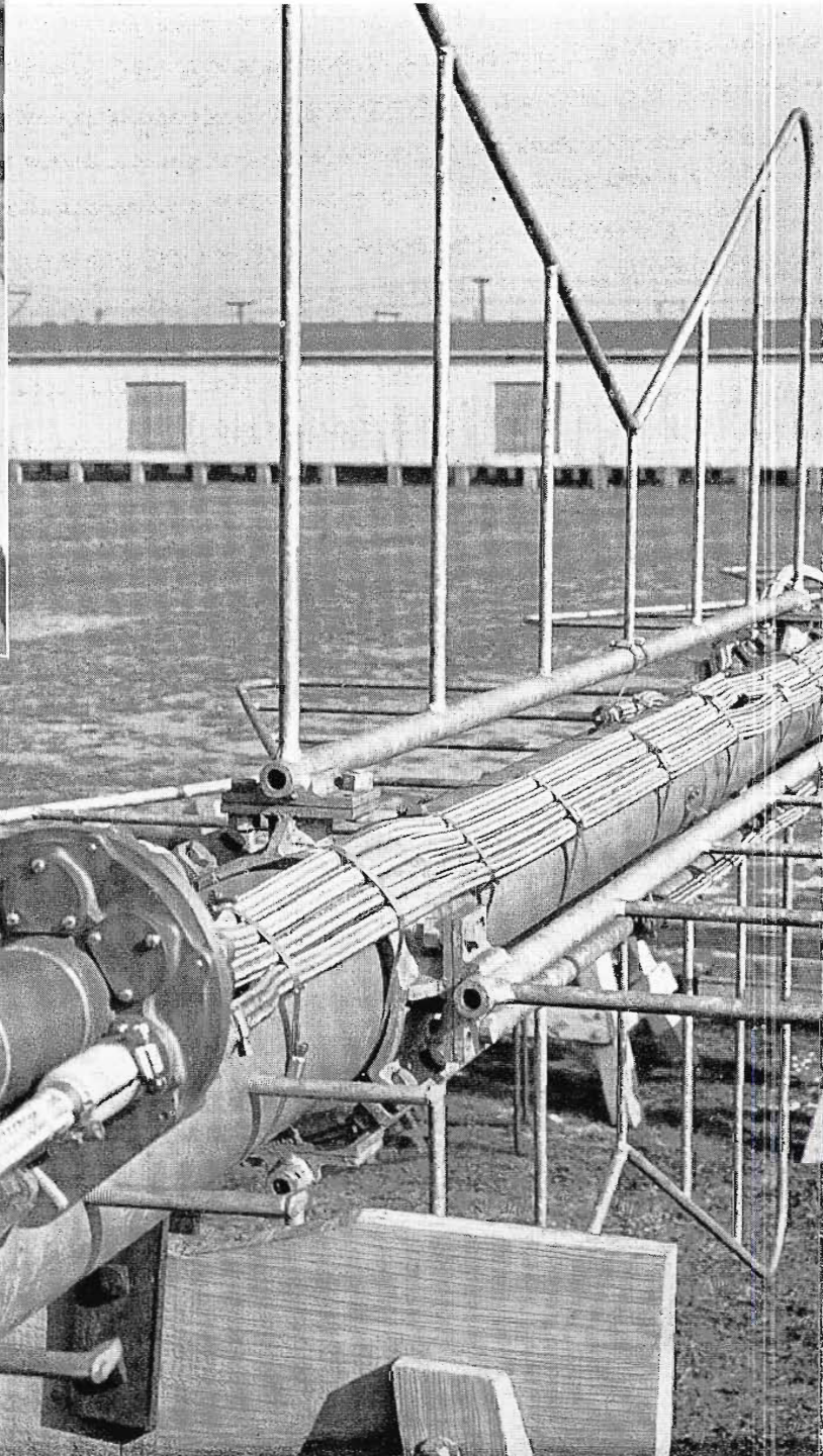
Below is a view of the upper two bays of the Channel 4 Super Turnstile antenna placed on trestles for wiring. Junction boxes mounted on opposite sides of pole receive the RG-35U cables from the eight sections (two for each bay, North-east and South-west). Flanged section below junction box is an impedance transformer.
