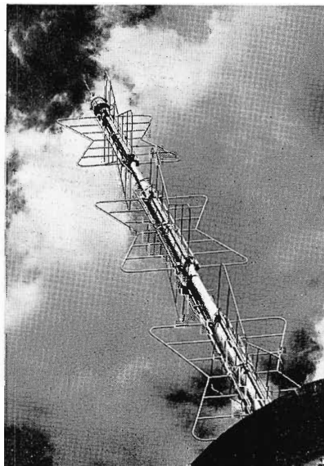
FIG. 1. Closeup of XHTV's Super Turnstile Antenna which tops Mexico City's skyline.
