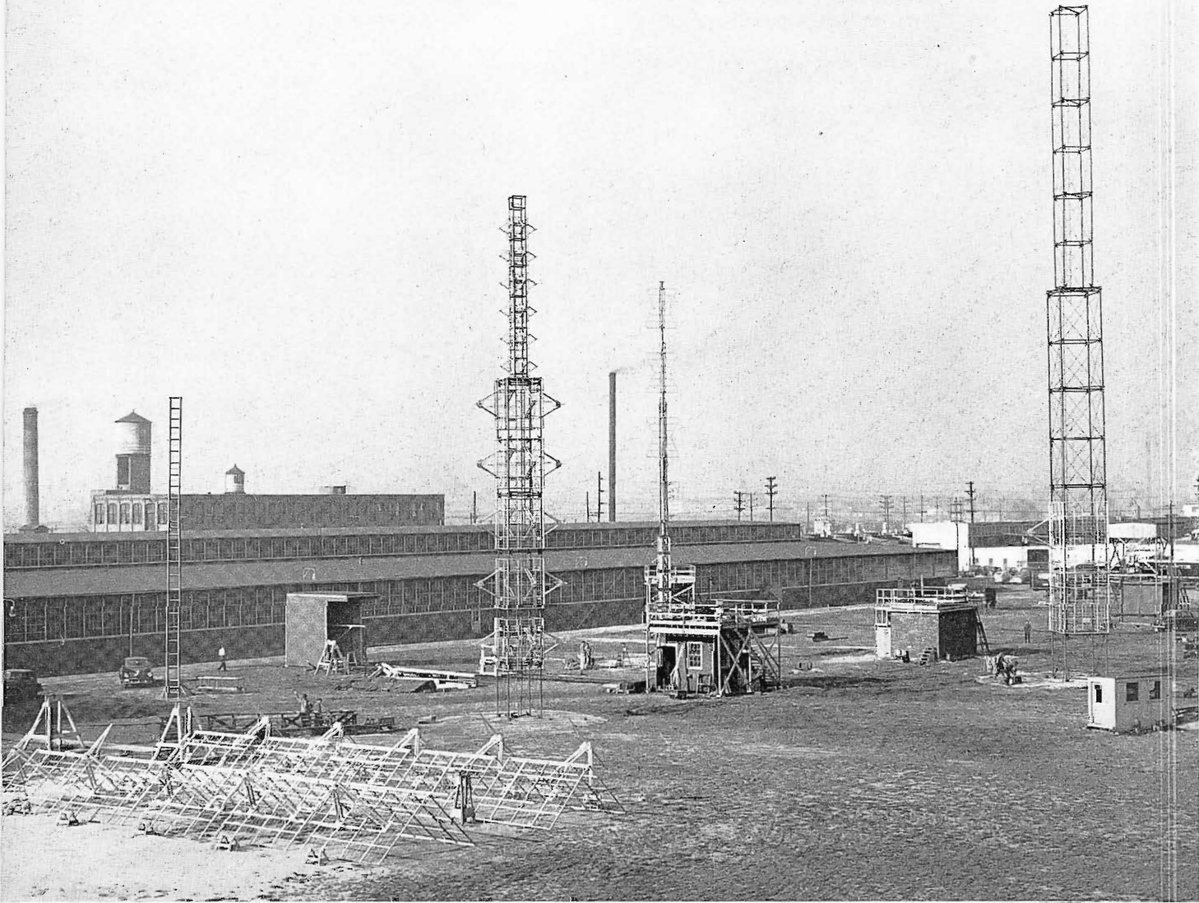
View of the RCA antenna test grounds at Camden showing towers which were erected especially for the Empire State antenna tests. Radiating elements are assembled on the towers and adjusted for minimum interaction and feed line SWR. Elements in the foreground are those of WCBS-TV.
