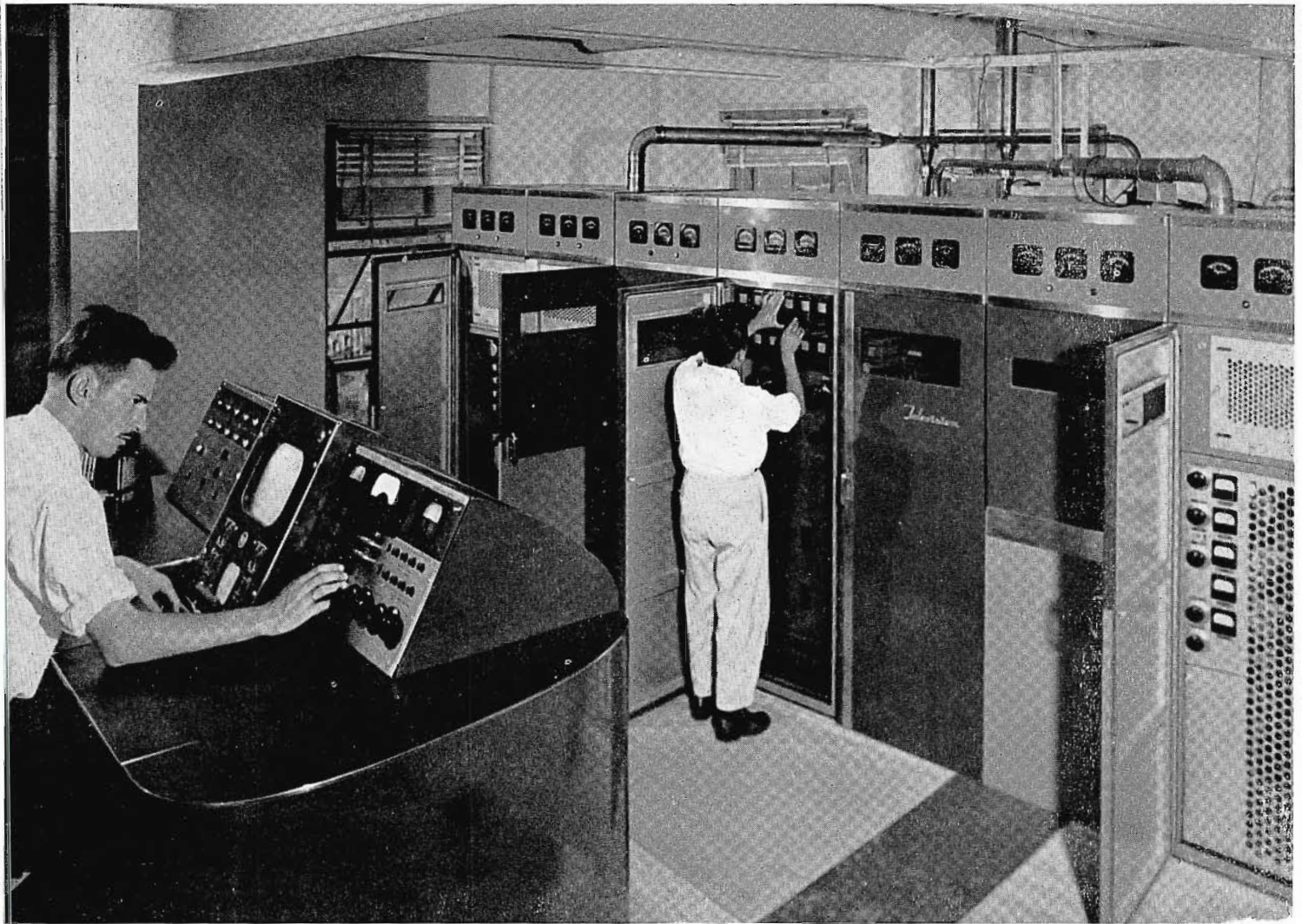
FIG. 12 (above). View of XHTV's 5-kw Television Transmitter (RCA TT-5A) and Transmitter Master Control Console.
