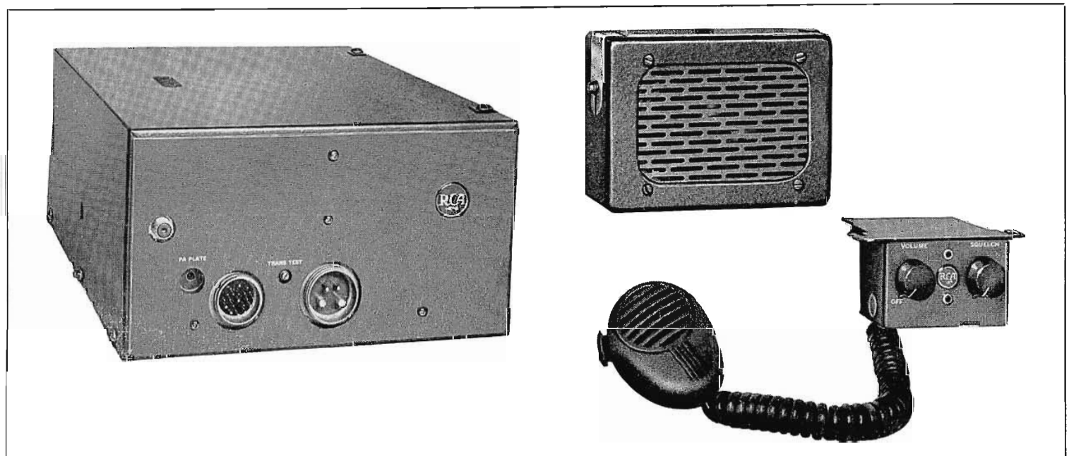
FIG. 9. The 30 watt Carfone, shown below, is a compact transmitter-receiver built into a single steel case which can be mounted in any convenient place in the vehicle. The loudspeaker, microphone, control unit and an antenna unit (not shown), are provided with the equipment.
