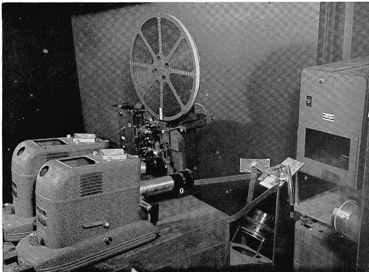
FIG. 5 (below). Corner-view of the KSD-TV Film Projection room showing the film projector and multiplexing system.
