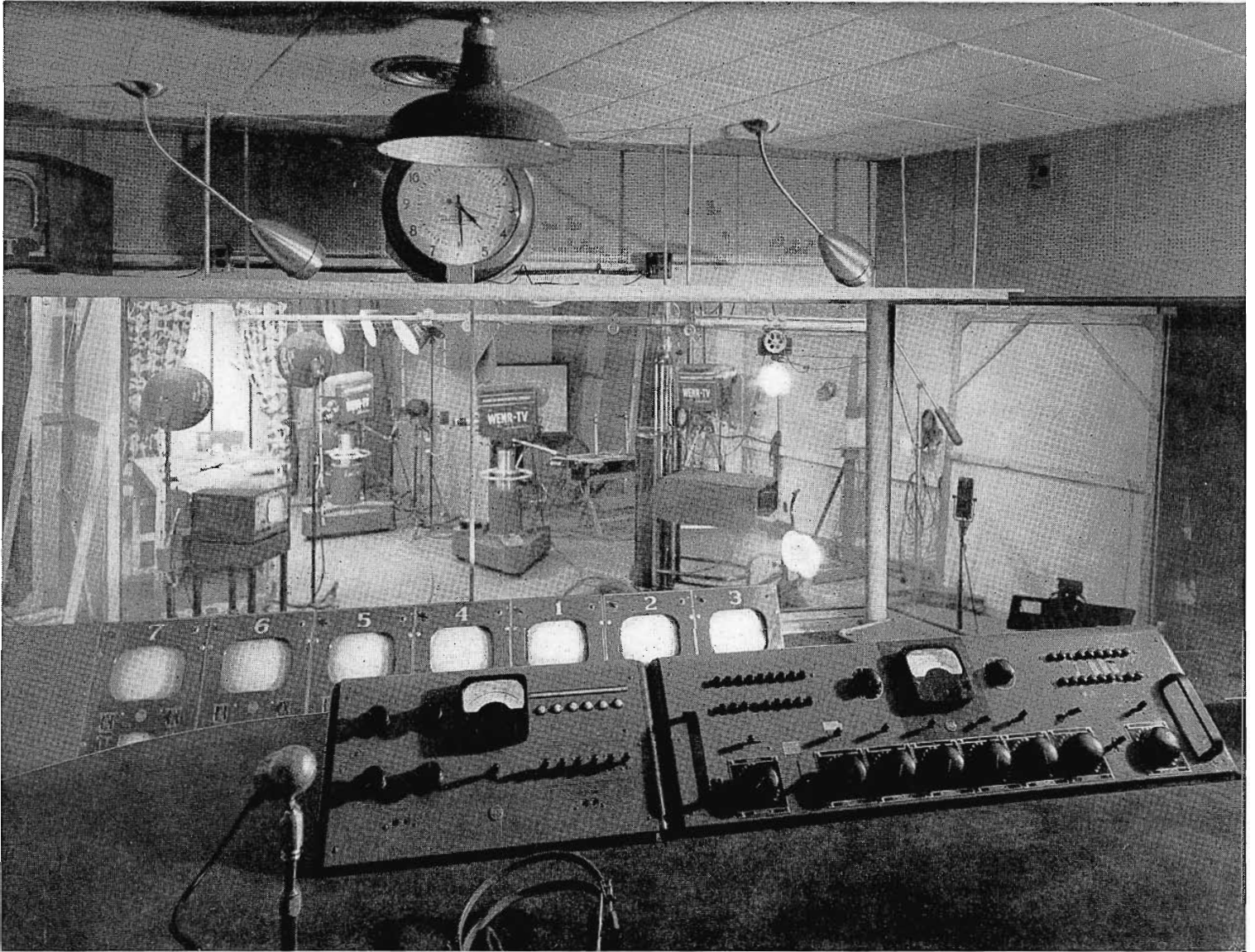
FIG. 3 (above). A typical station installation (photo by courtesy of WENR-TV) employing the audio system shown in Fig. 4. The audio units are located on a higher level, in order that the audio operator has visible access to the studio and video monitors.
