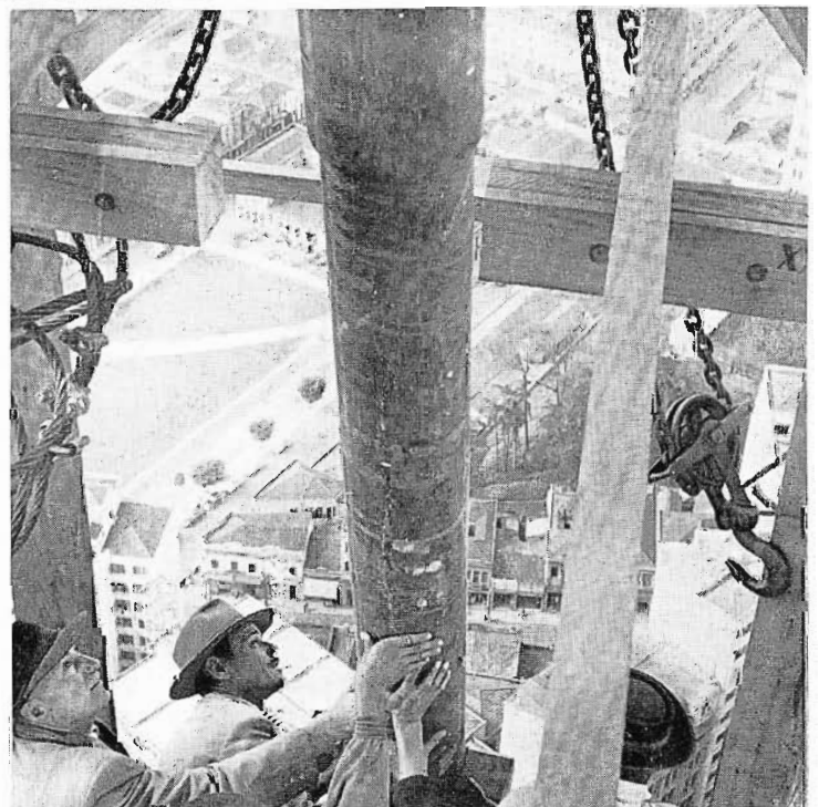
FIG. 24 (below). In this view, the PRF3-TV antenna is shown being lifted to the top of the tower on the Sao Paulo State Bank Building.
