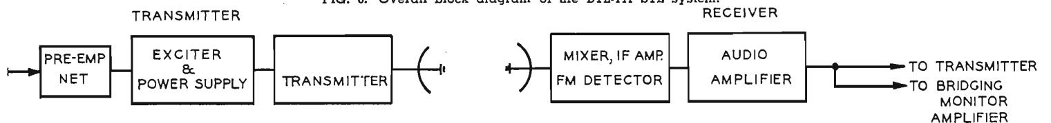
FIG. 3. Overall block diagram of the BTL-1A STL system.
