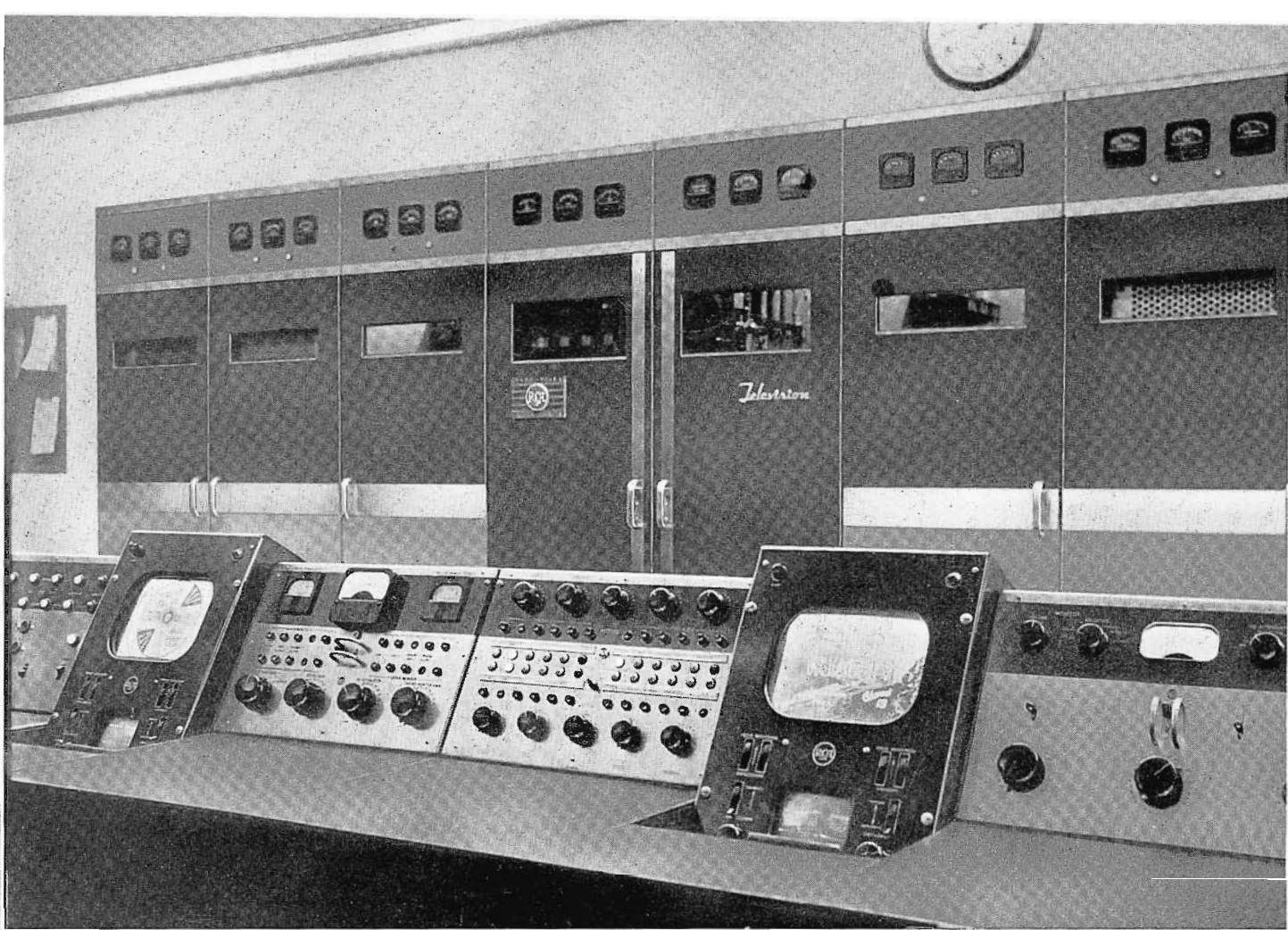
Photo above gives a better view of the FM-TV transmitter console, and TV program switching turret (center of photo). FM turret is at extreme right, TV transmitter monitor and control turrets at left. Right hand monitor unit is for program preview.
