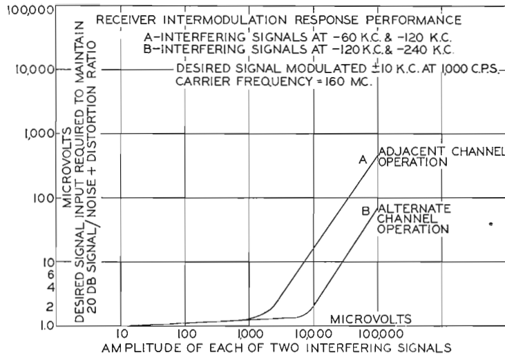
FIG. 16. Receiver intermodulation rejection.
