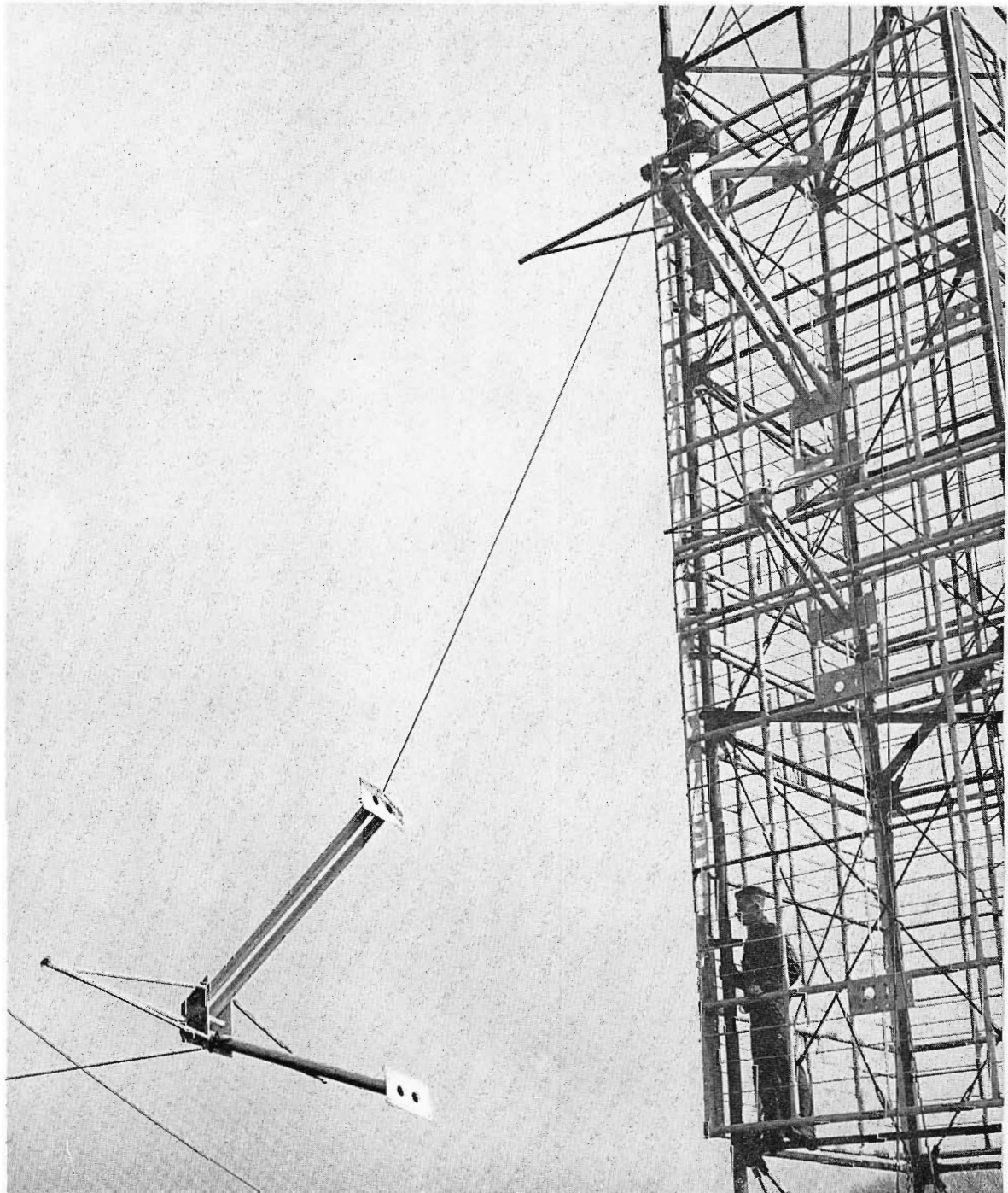
A. Channel 2 dipole being hoisted into position for assembly to the backing screen on the tower. Note WCBS-FM dipole installed between the TV elements. The FM signals of WJZ-FM and WNBC-FM will also be radiated from the Empire State tower.
