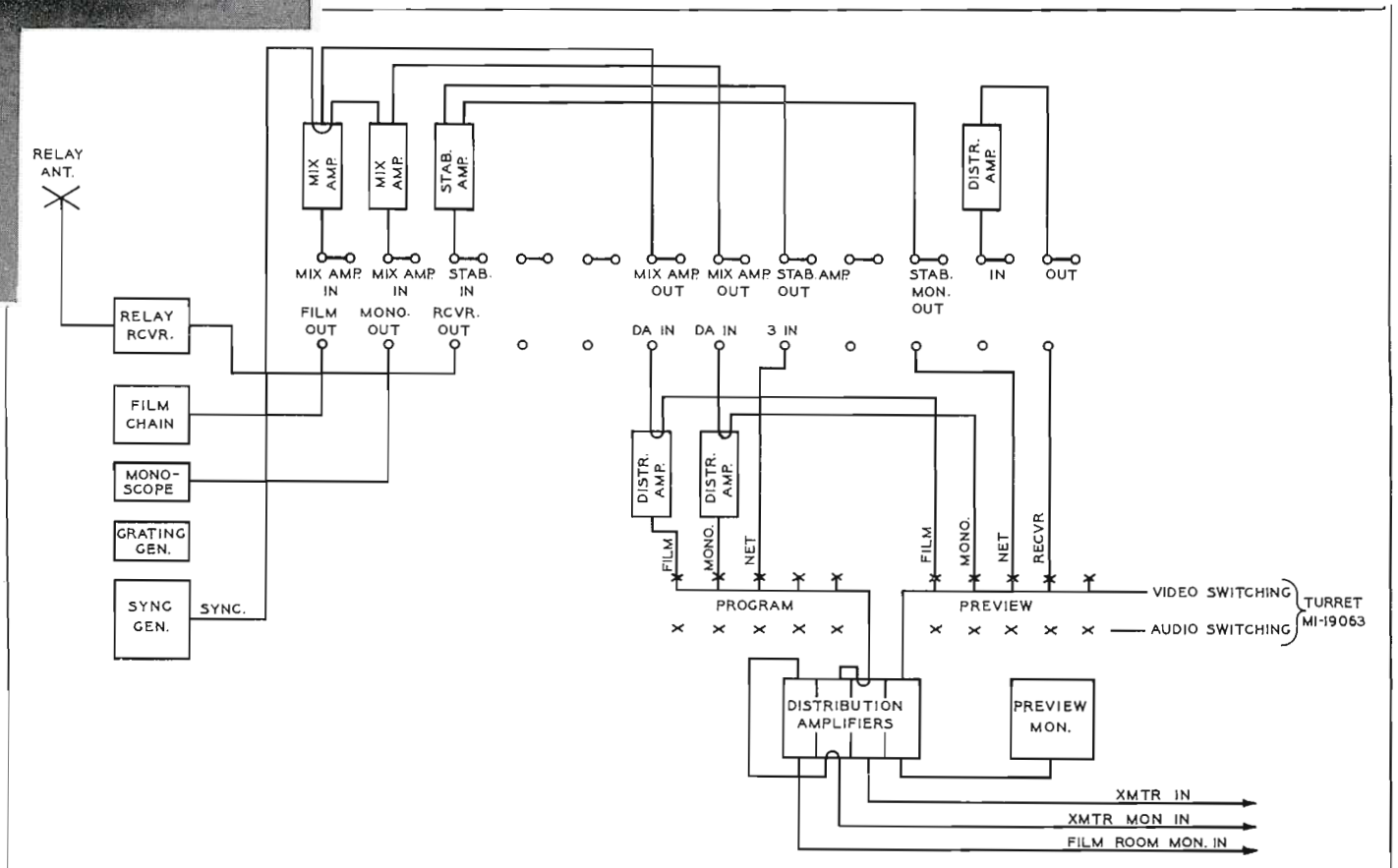
Block diagram of WJAC-TV video facilities. Turret MI-19063 is the program switching unit which is mounted in the transmitter control console. Other connections not shown on the diagram are the network line from AT & T, and a line from the grating generator.
