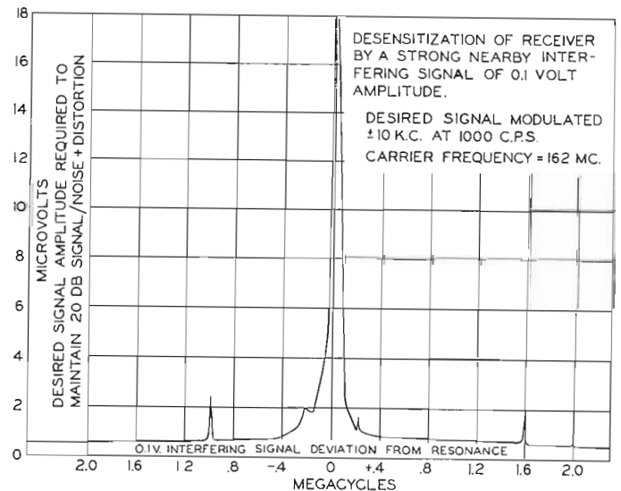
FIG. 15. Receiver spurious response rejection.
