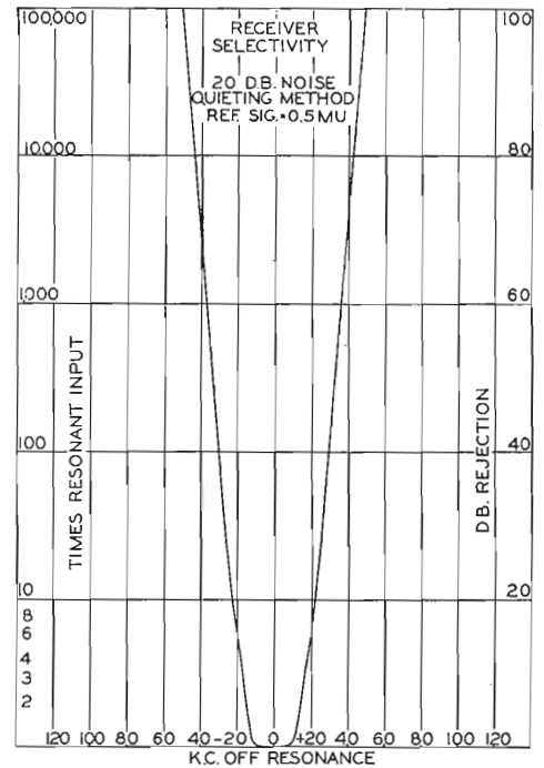
FIG. 13. Receiver selectivity.
