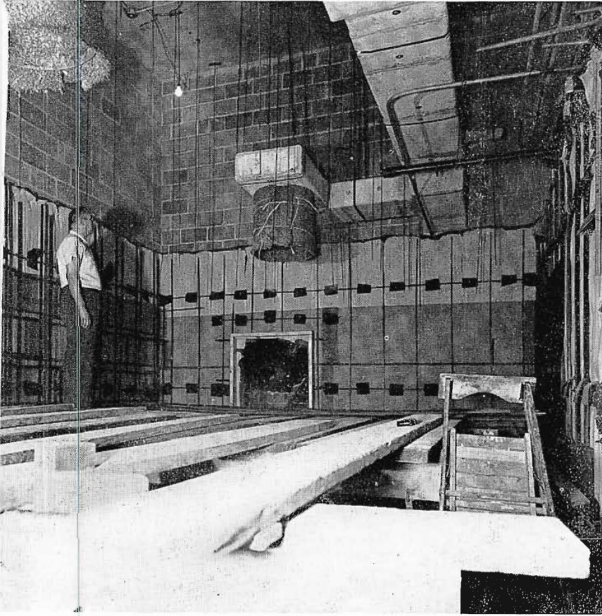
▲ FIG. 6. This photo shows how the studio ceiling is specially suspended by wires for best acoustical properties.
