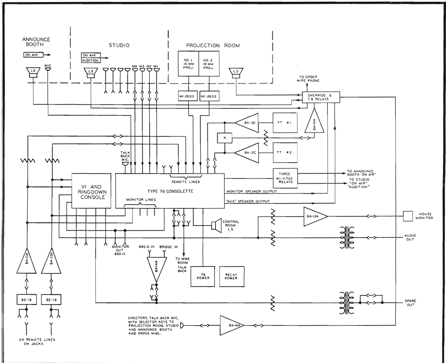
FIG. 4 (below). Single line block diagram of a flexible TV audio system for one studio, announce booth, remote lines and film projection room.
