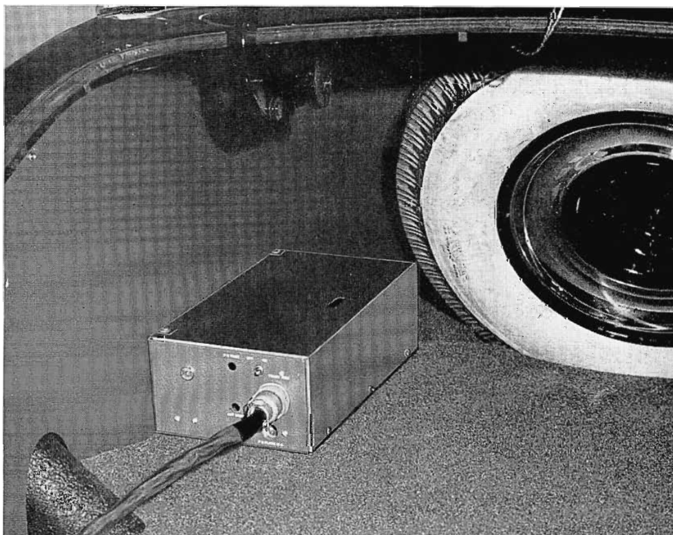
FIG. 12. RCA two way radio communications equipment takes up very little space in car trunk. It mounts in space behind the spare tire, as shown, and is very easily available for servicing.
