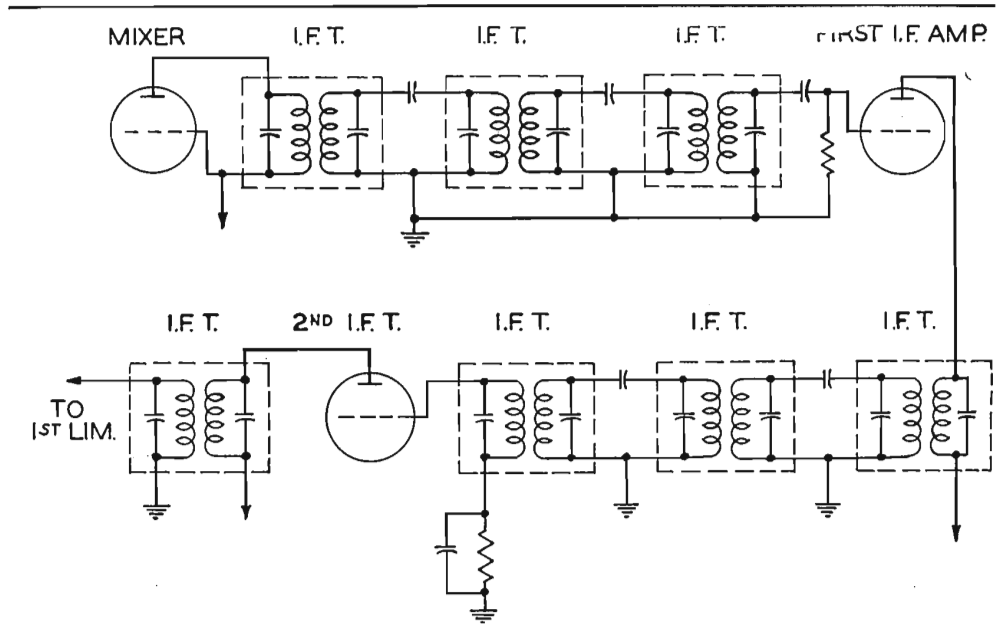
FIG. 8 (at right). Schematic shows a portion of the receiver intermediate frequency amplifier.
